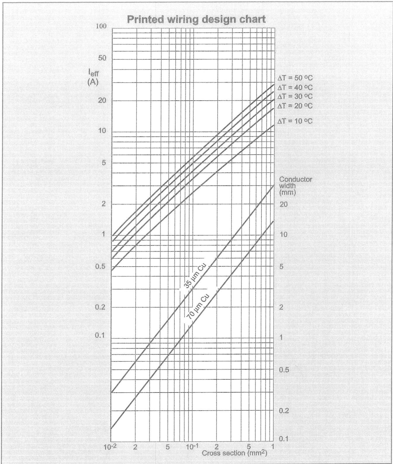
Fig.2 Relation between current, dimensions of tracks in PCBs and temperature rise.
