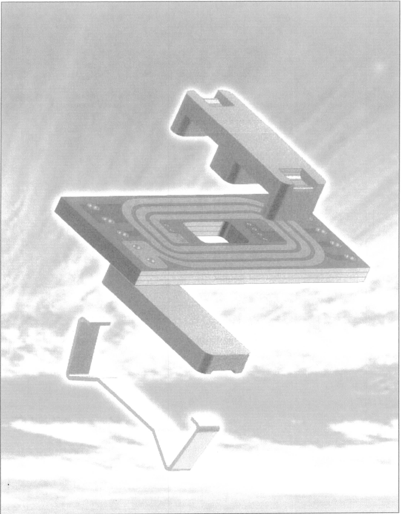
Exploded view of a planar transformer
